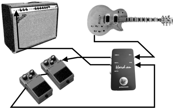
EFFECTS PEDAL HARD BYPASS Guitar to IN A : THRU A to Pedal input : Pedal Out to IN B : OUT A to Amp input
