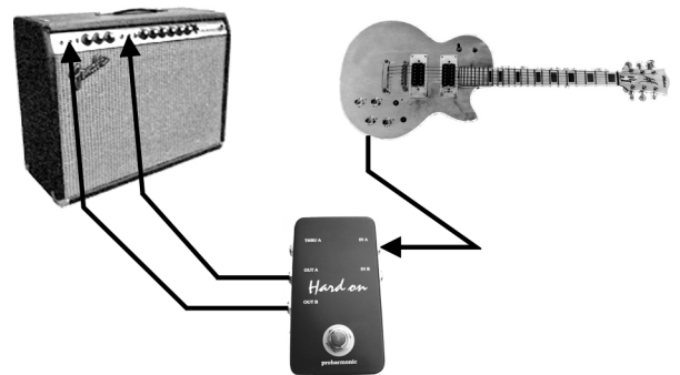
AMPLIFIER OR AMPLIFIER CHANNEL SELECT Guitar to IN A : OUT A to Amp input 1 : OUT B to Amp input 2
