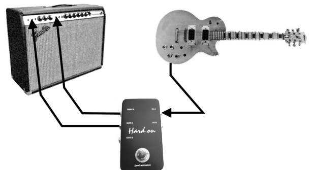
AMPLIFIER CHANNEL ADD Guitar to IN A : THRU A to Amp input : OUT A to second Amp input
